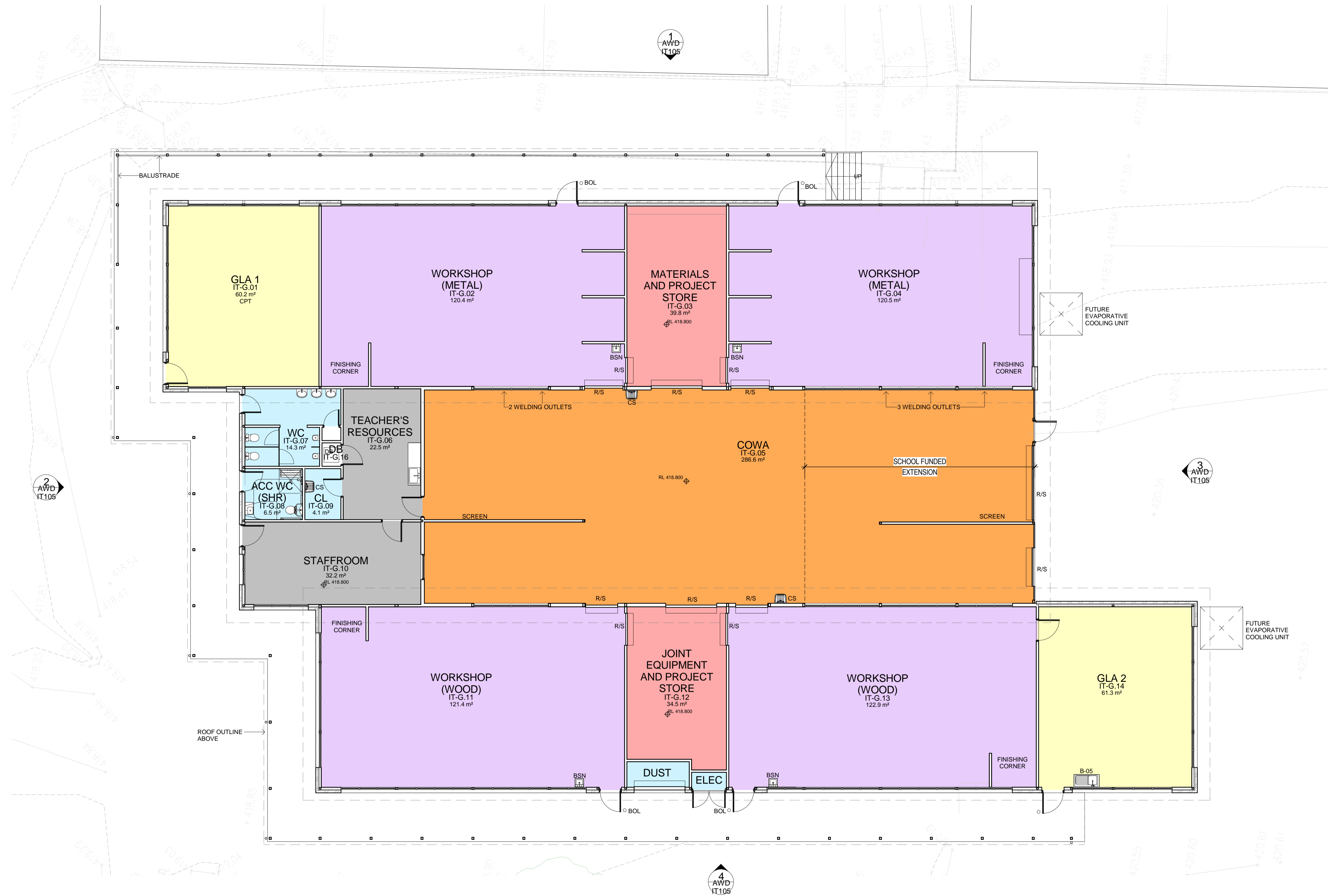
1 Industrial Tech Building - Floor Plan. 1 : 100
