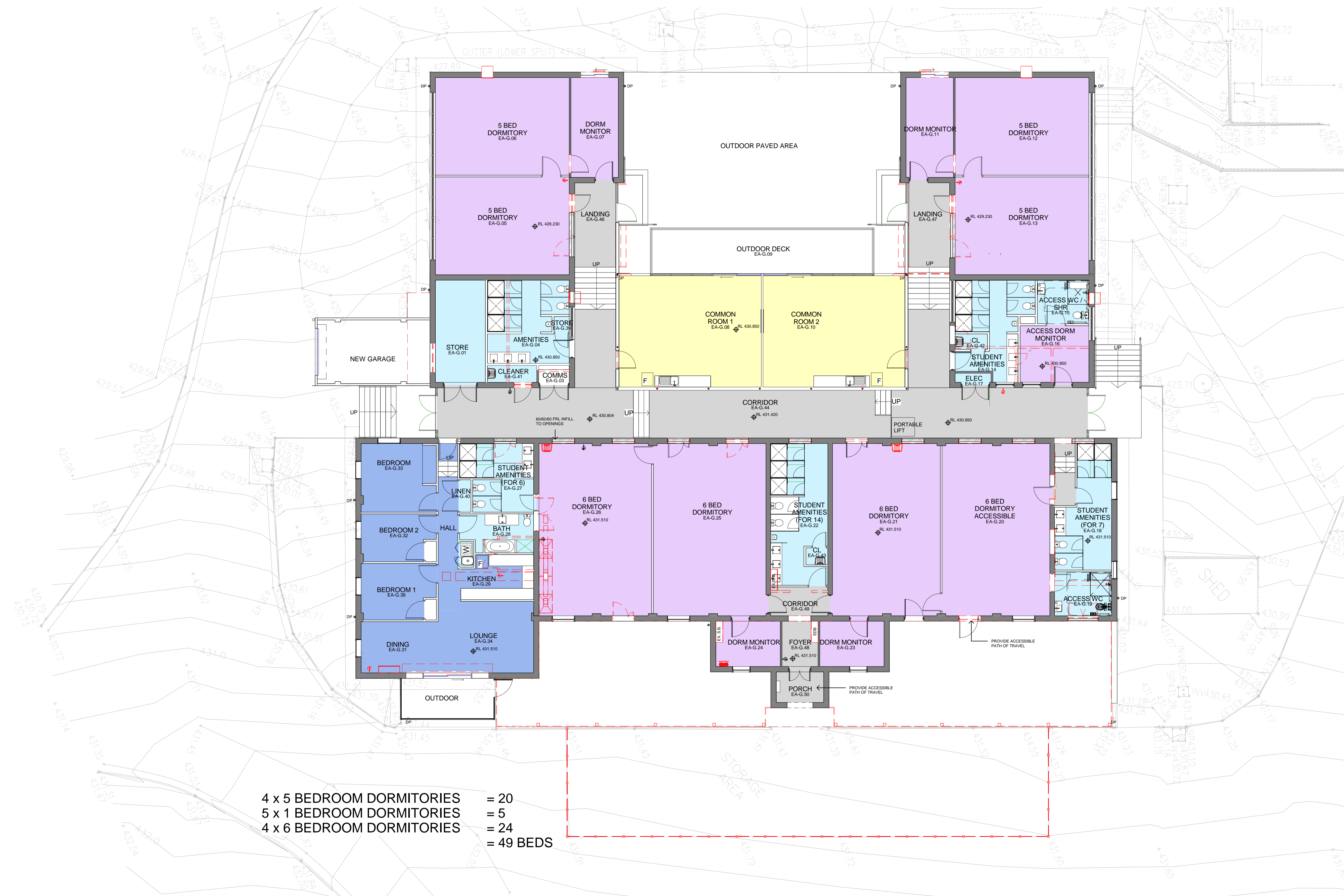
1 Block EAWK - Ground Level. 1:100
